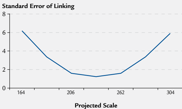
Figure 15: Standard Error of Linking Curve for Mathematics Grade 4
