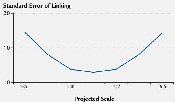
Figure 16: Standard Error of Linking Curve for Mathematics Grade 8
